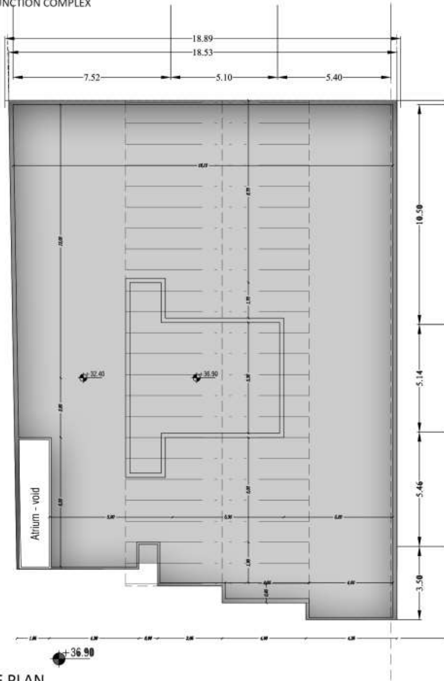
ROOF PLAN
