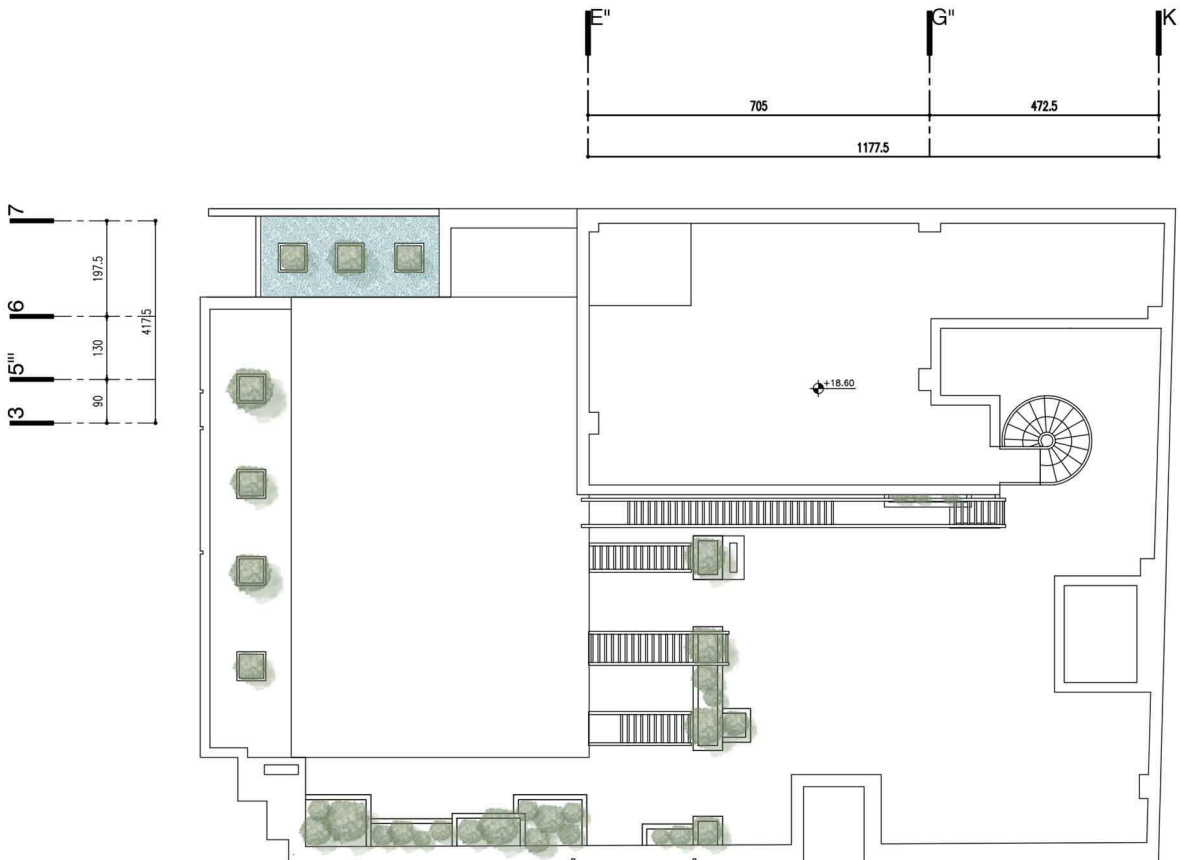
ROOF PLAN NOT TO SCALE
