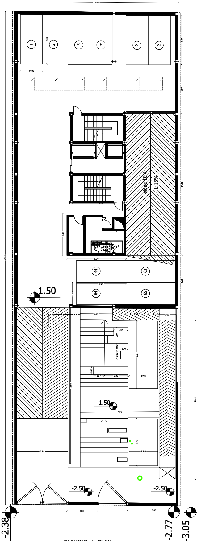
PARKING -1 PLAN
