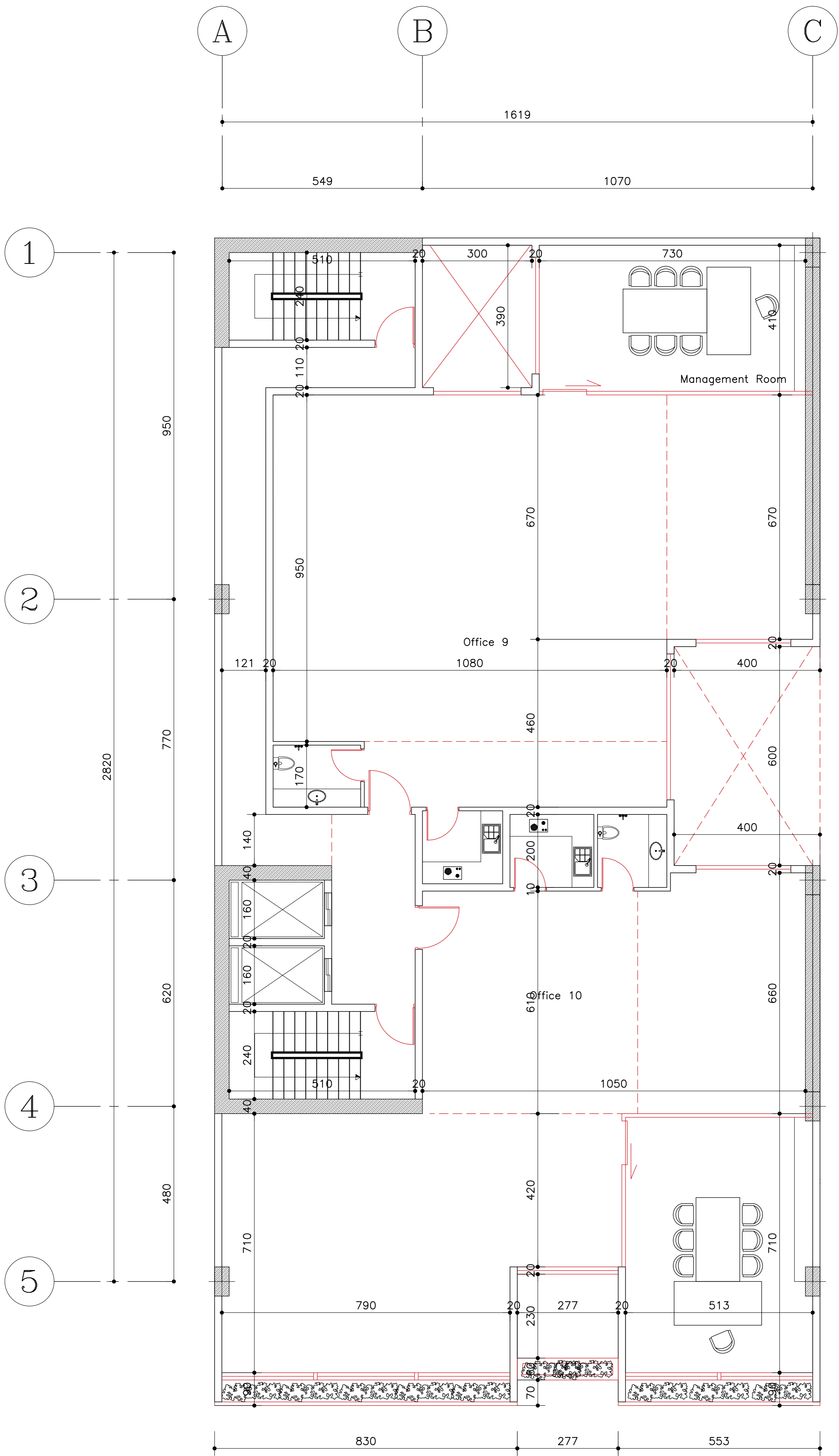
+4 FLOOR PLAN
