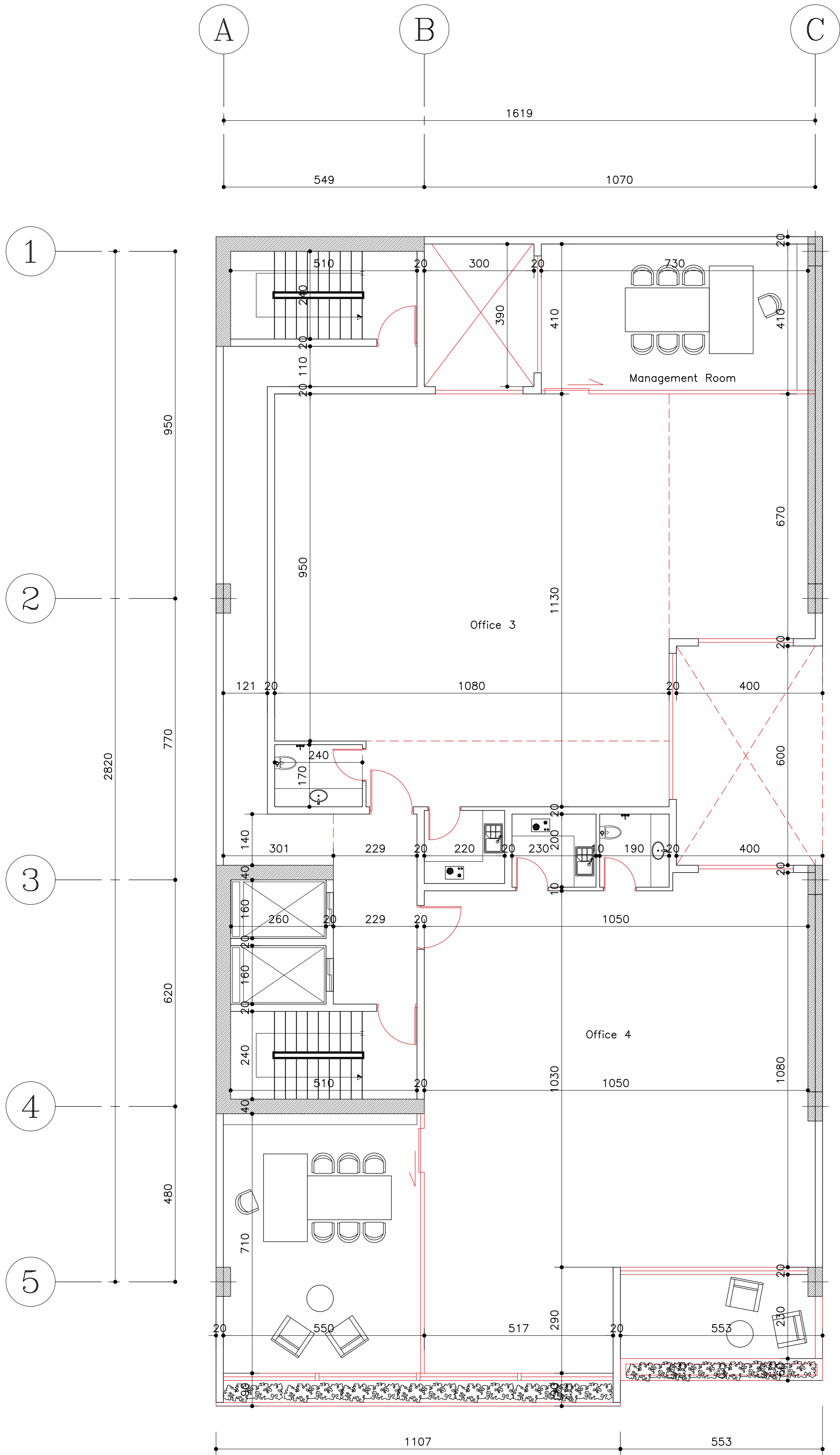
+1 FLOOR PLAN
