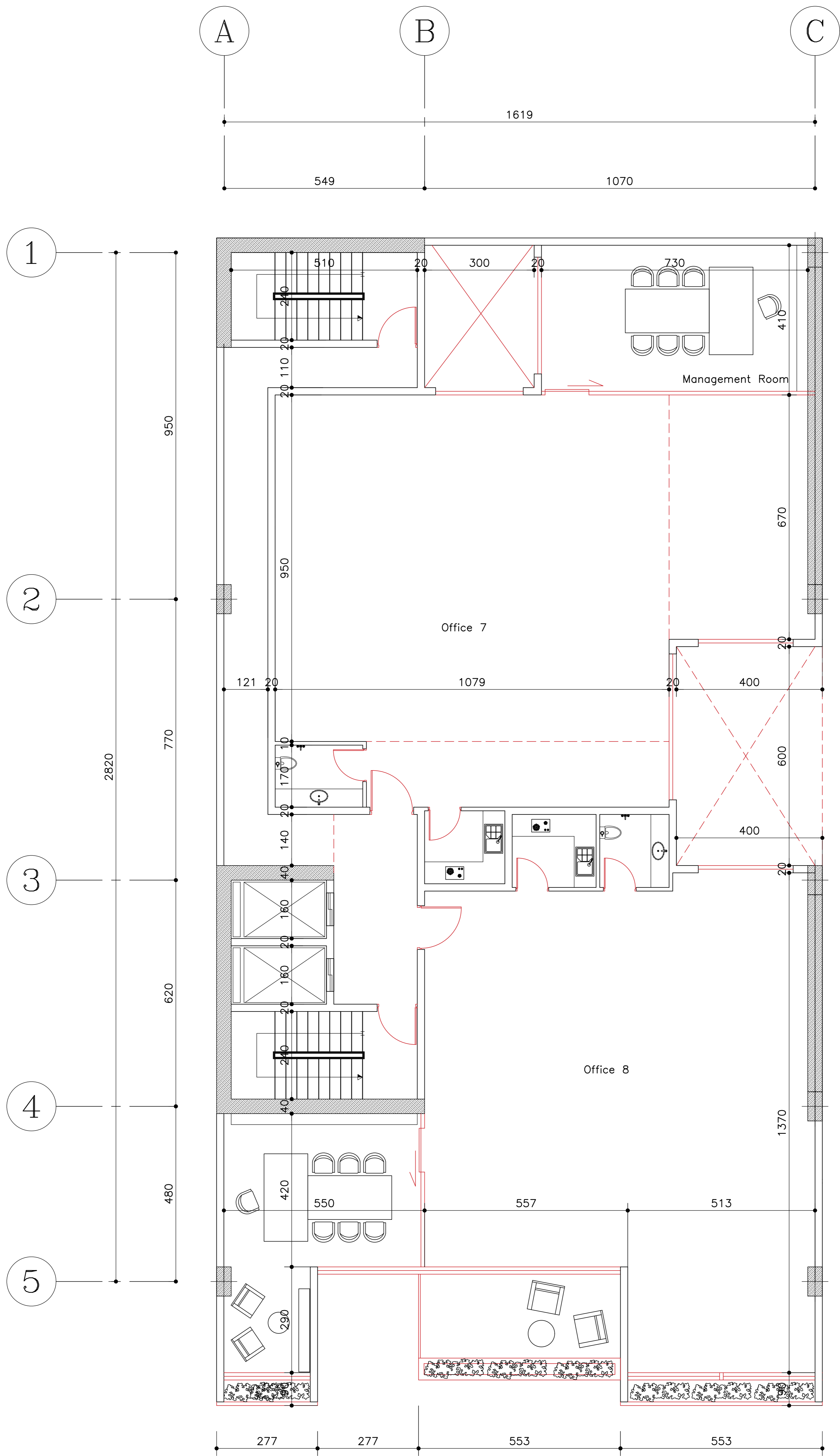
+3 FLOOR PLAN
