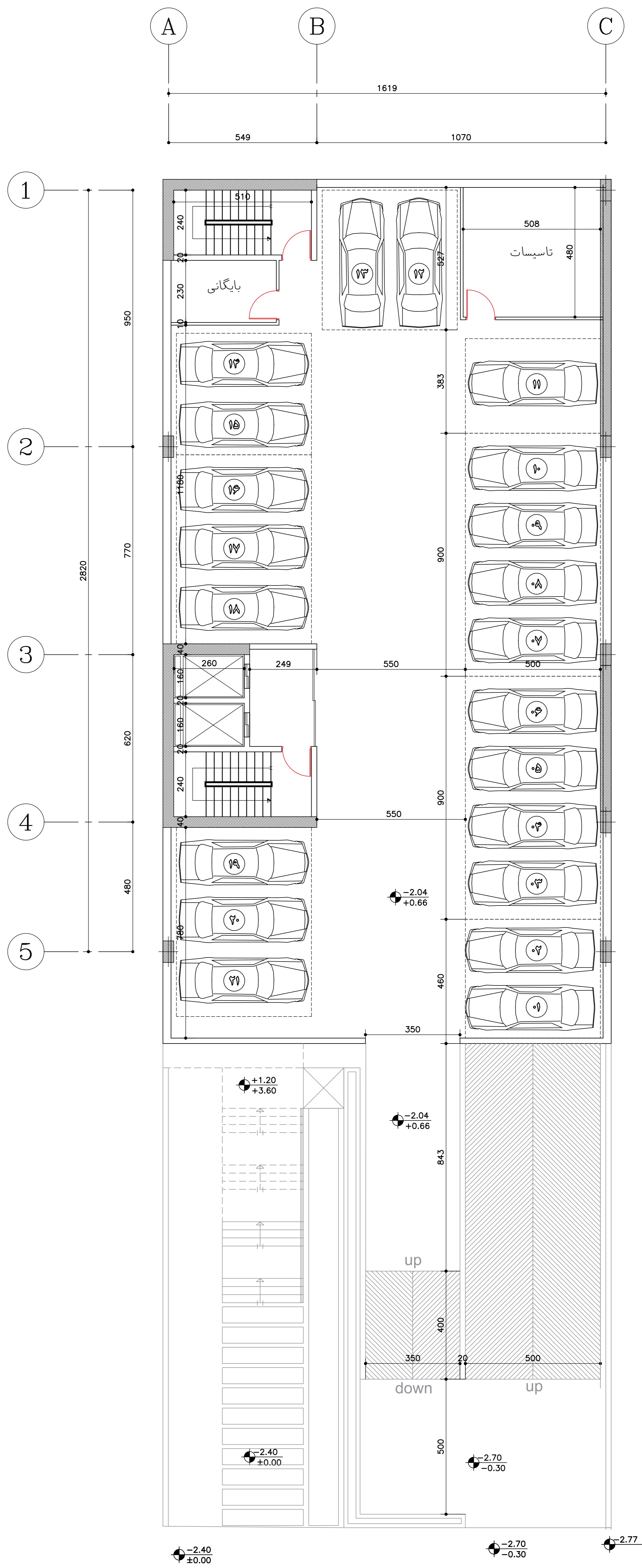
-1 Basement
