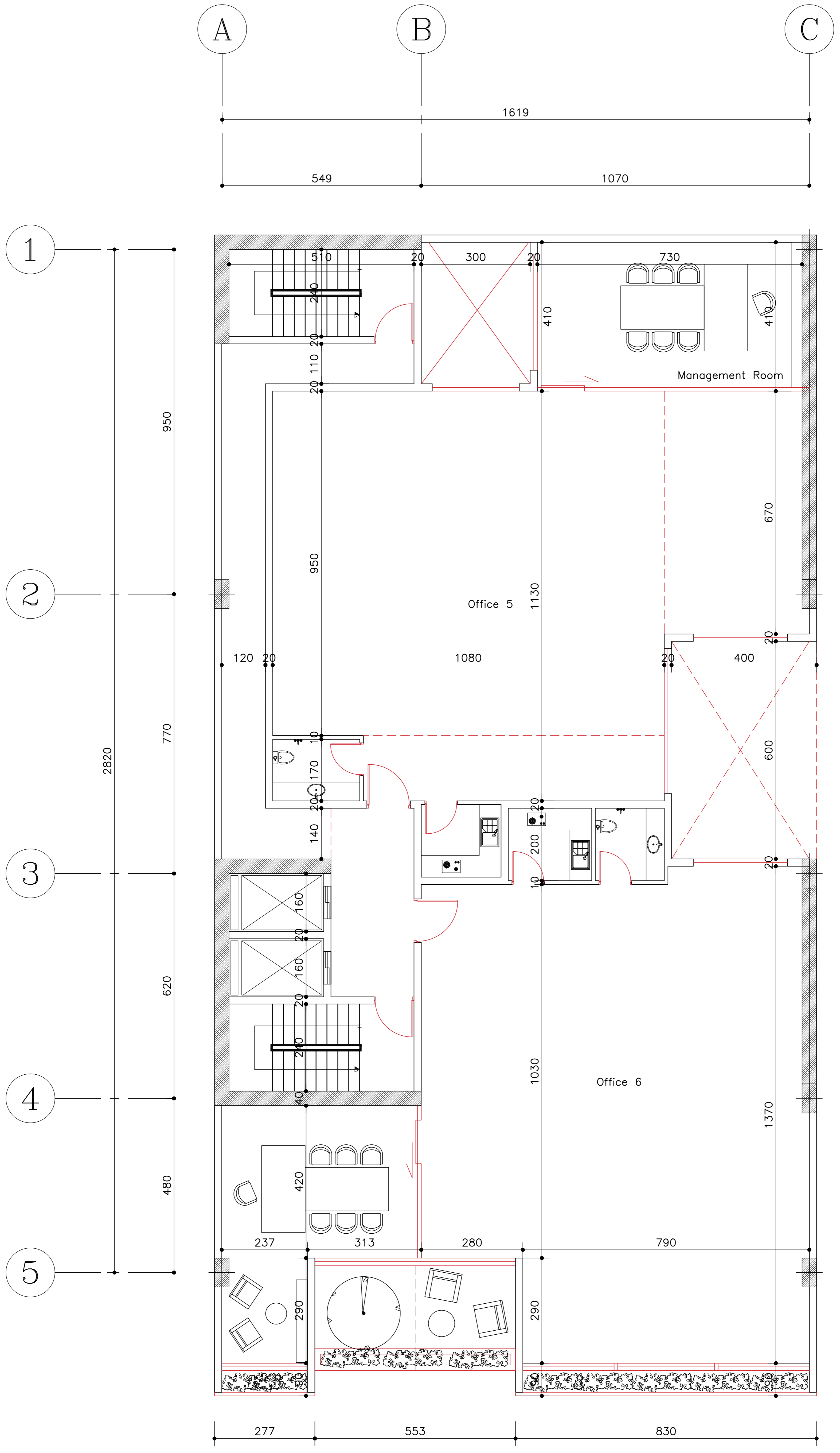
+2 FLOOR PLAN
