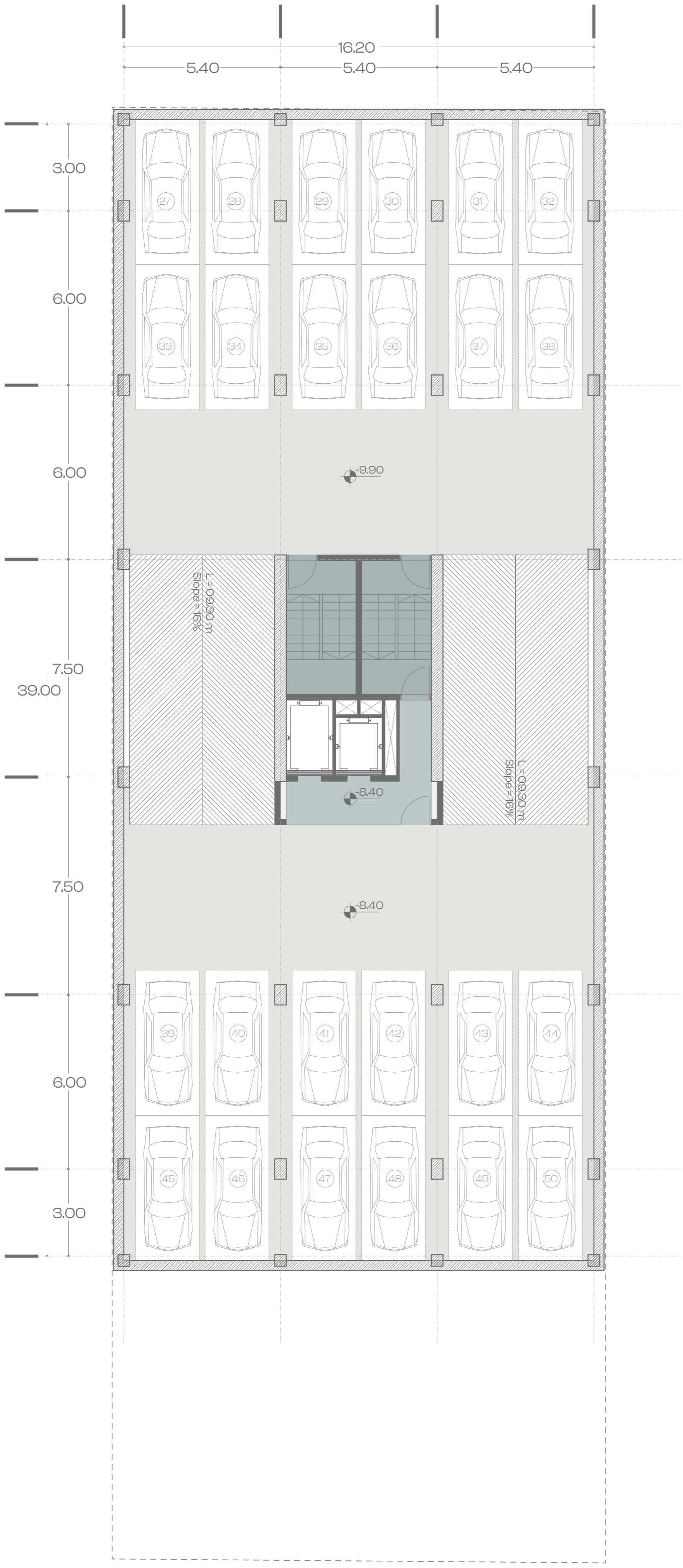
-3rd Basement Floor Plan Scale: 1/100
