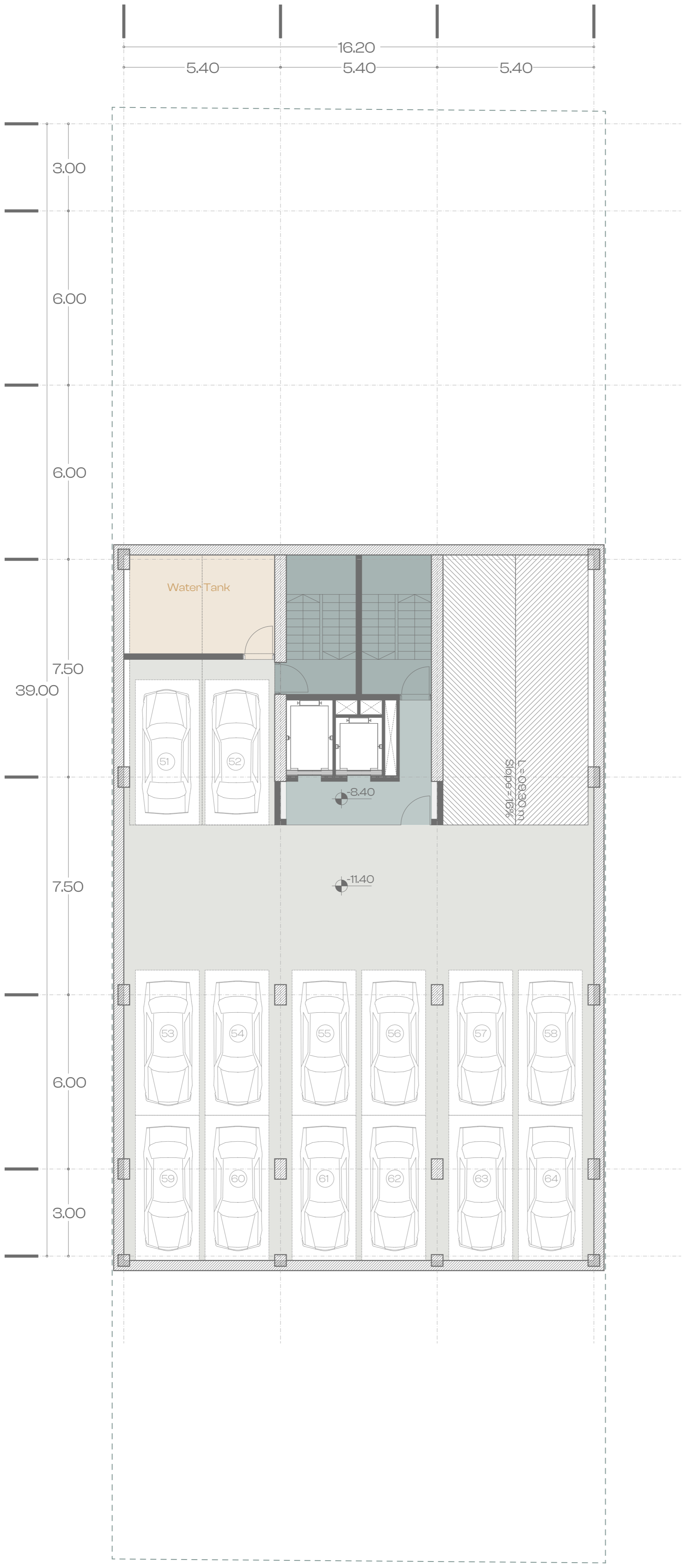
Alternative.A -4th Basement Floor Plan Scale: 1/100
