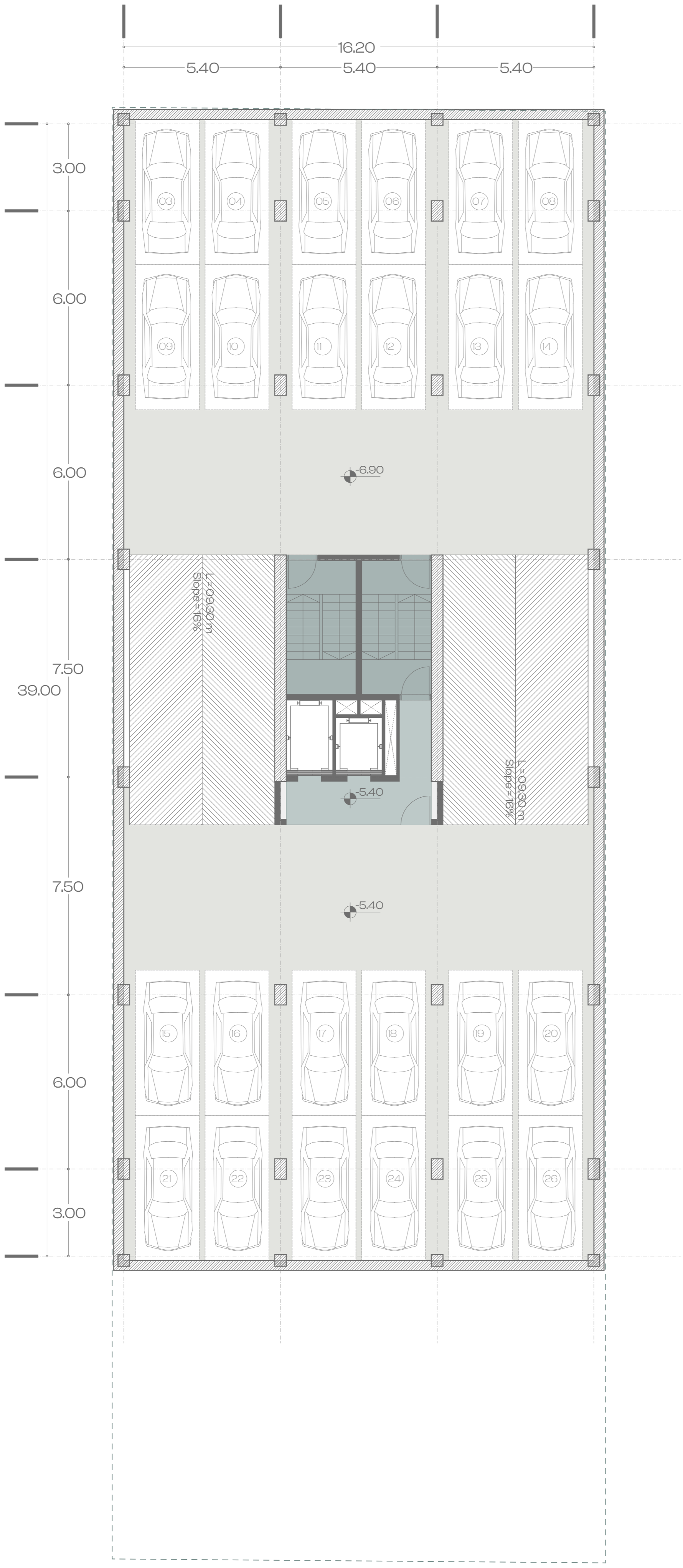
-2nd Basement Floor Plan Scale: 1/100
