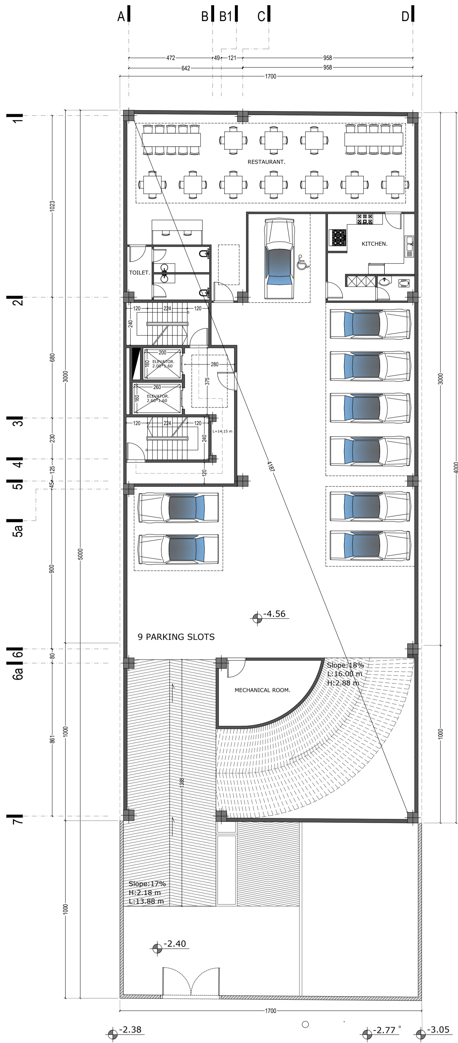
-2 Basement Floor Plan - Alt 2 (with restaurant)
