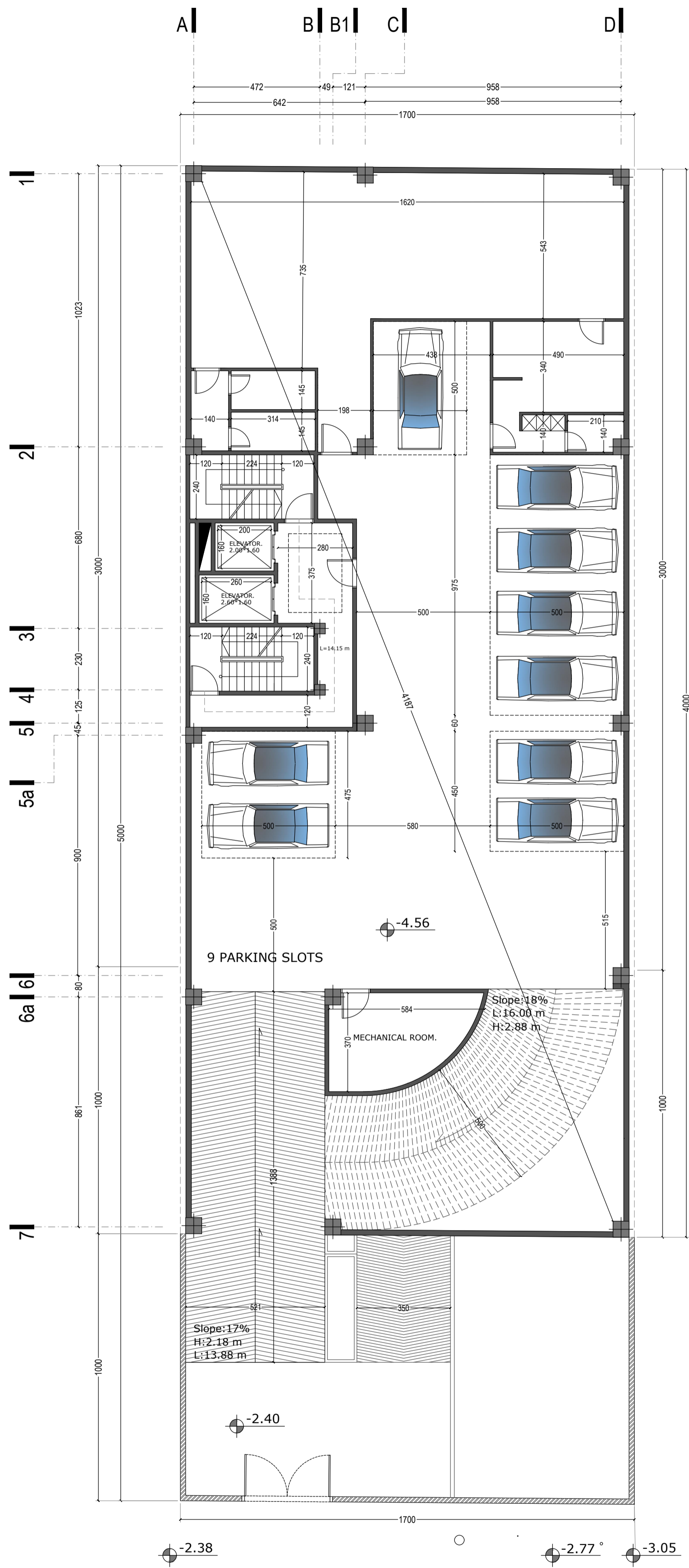
-2 Basement Floor Dimension Plan - Alt 2 (with restaurant)
