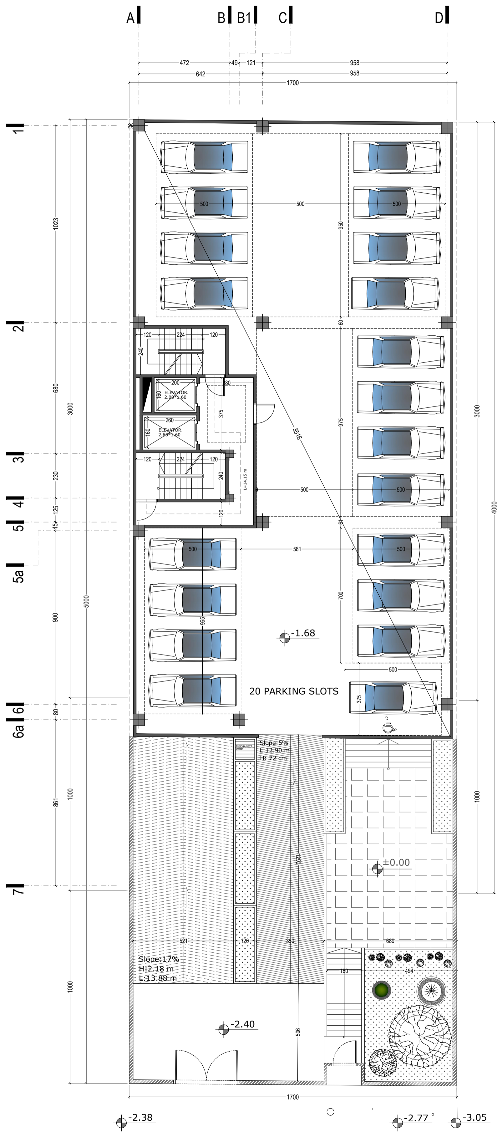
-1 Basement Floor Plan
