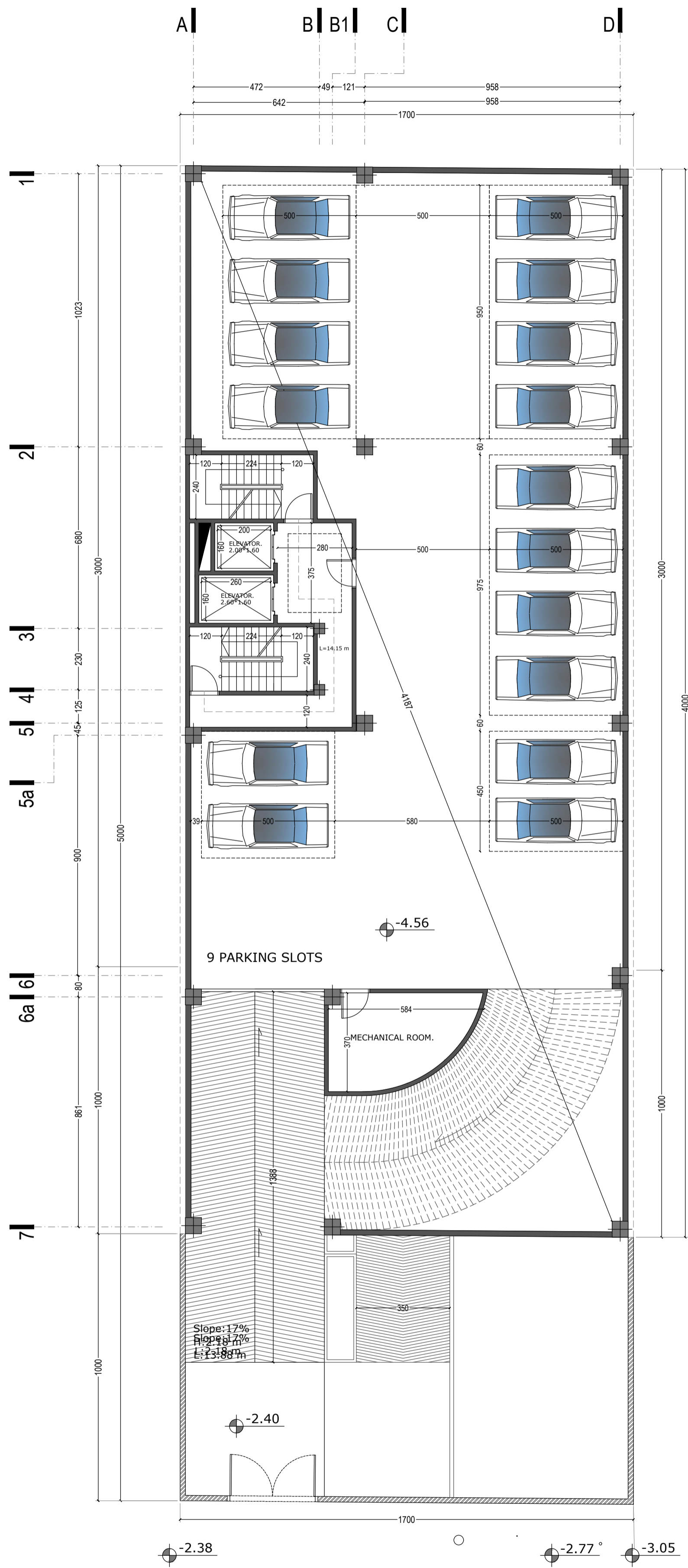
-2 Basement Floor Plan Alt1 (without restaurant)
