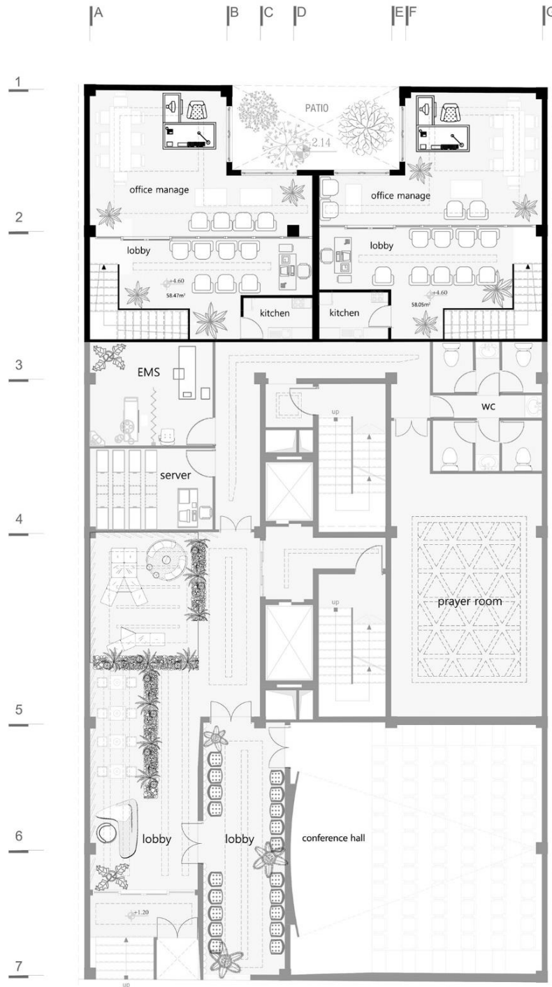
Ground floor duplex plan
