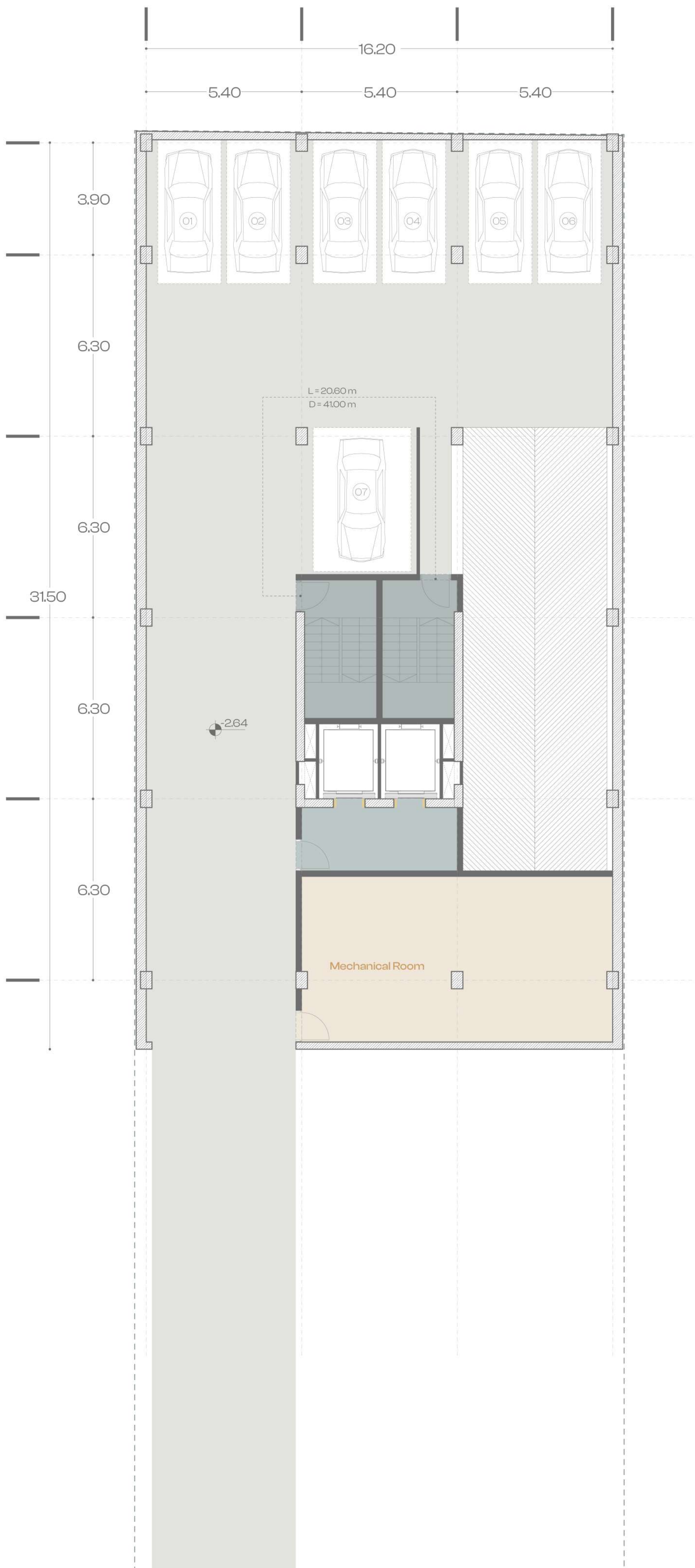
First Basement Floor Plan Scale: 1/100
