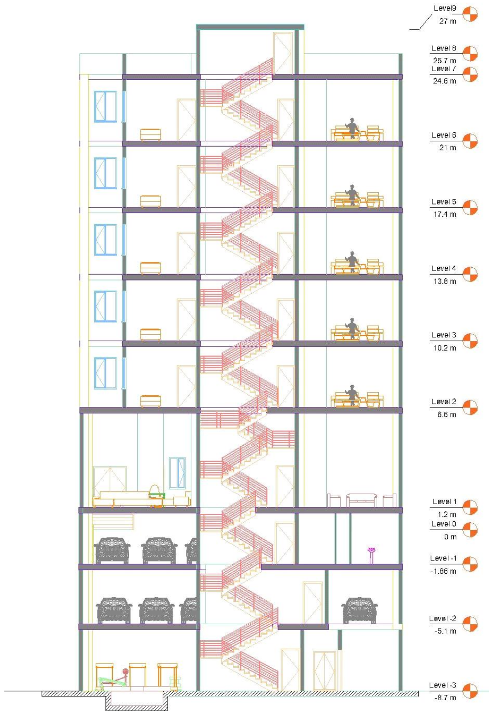
section B-B
