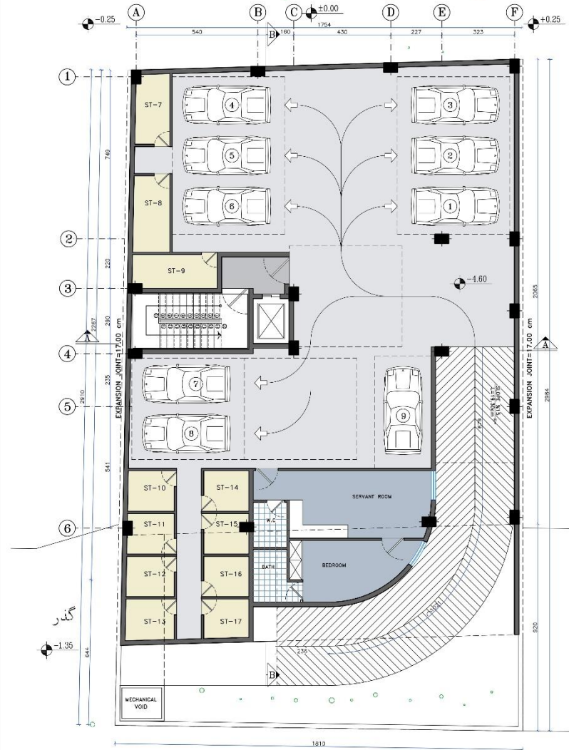
BASEMENT-2 FLOOR PLAN SC. 1:100
