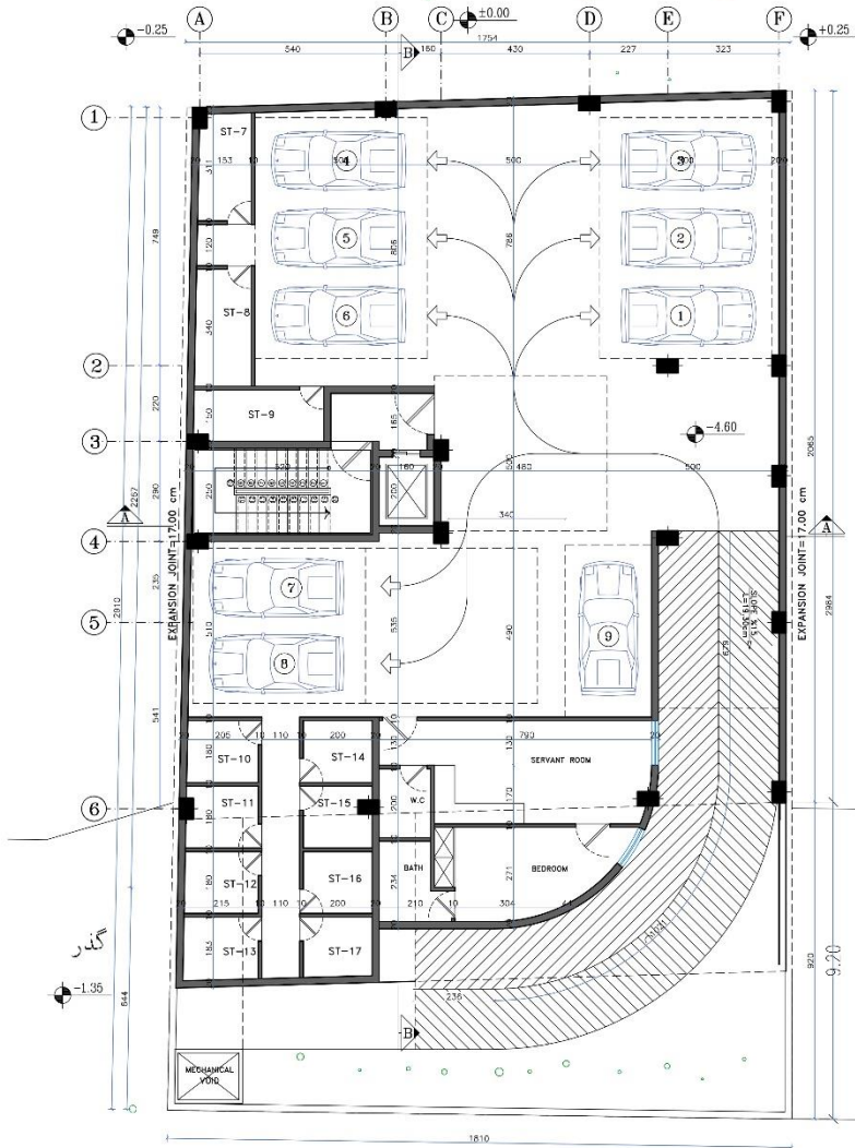
BASEMENT-2 FLOOR PLAN SC. 1:100
