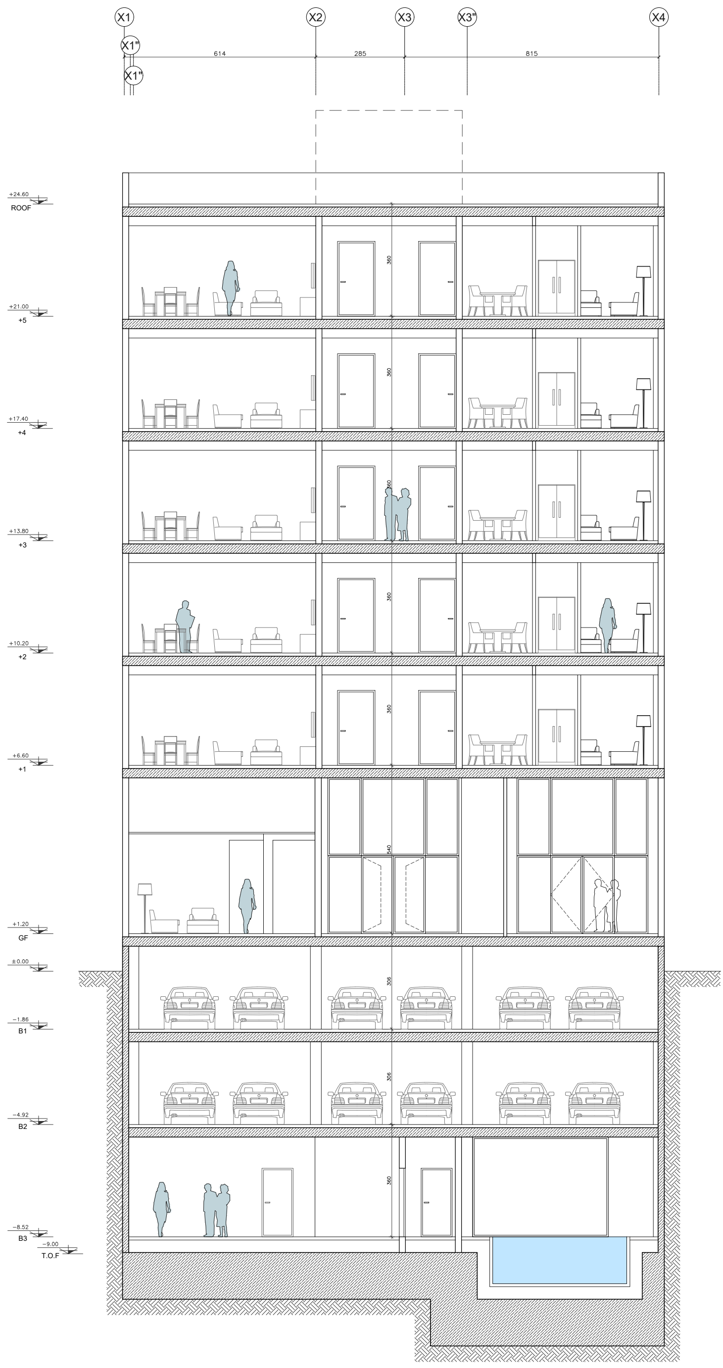
SECTION B-B
