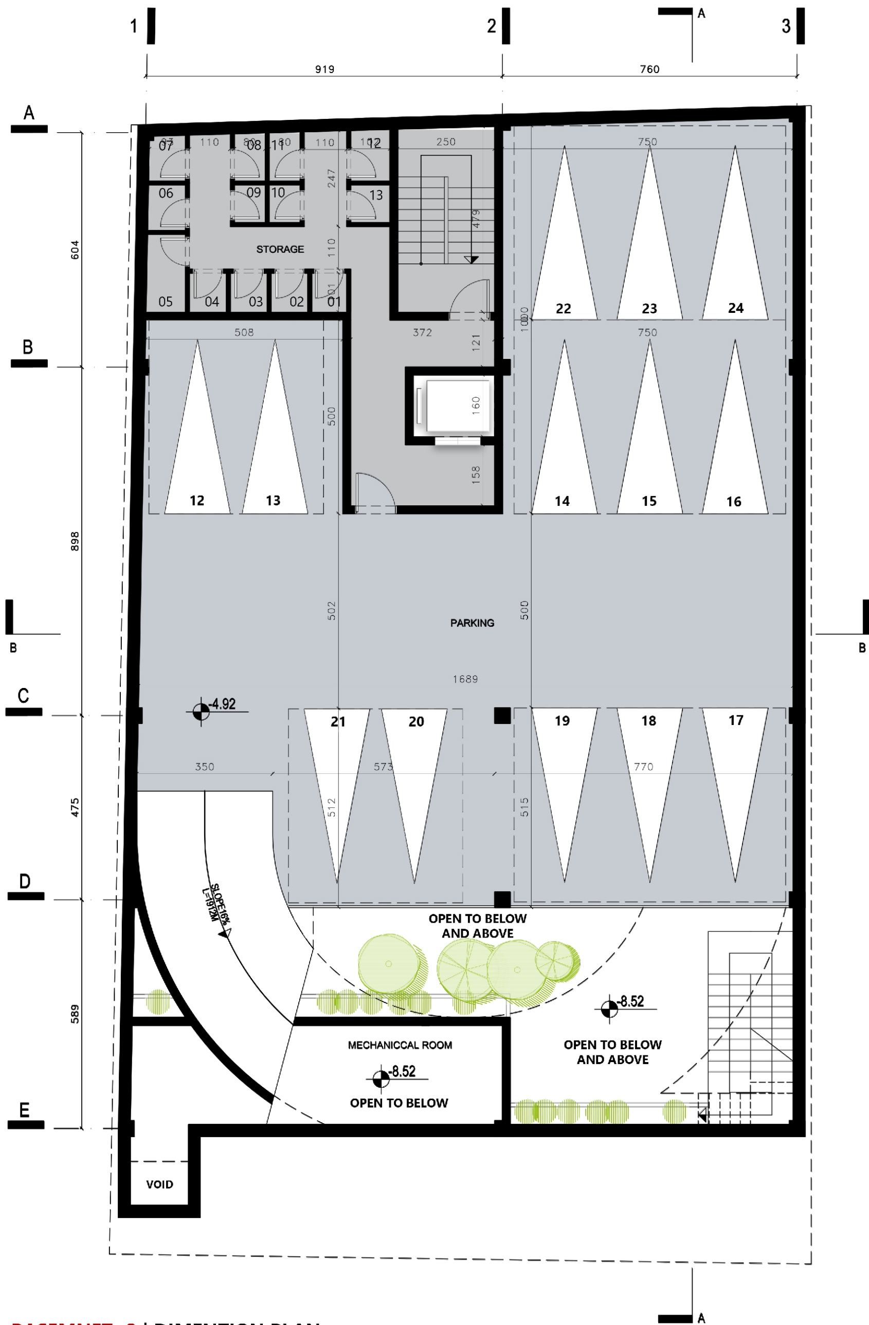
BASEMNET -2 | DIMENTION PLAN PARKING NO. 13
