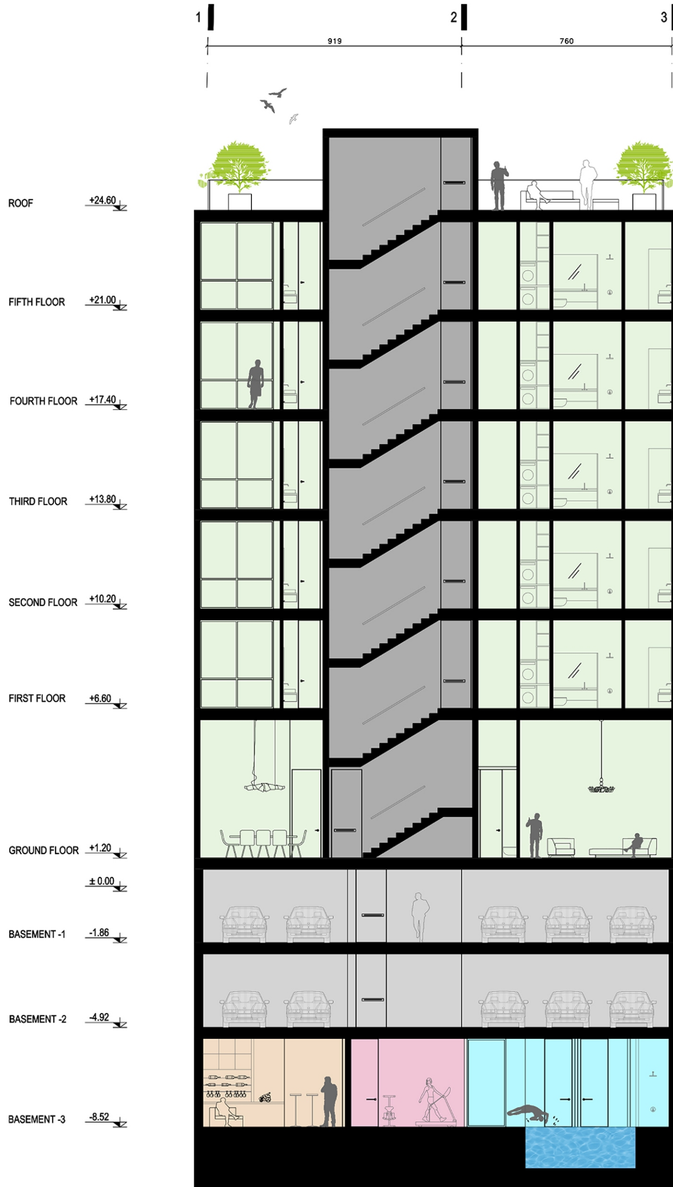
SECTION B-B
