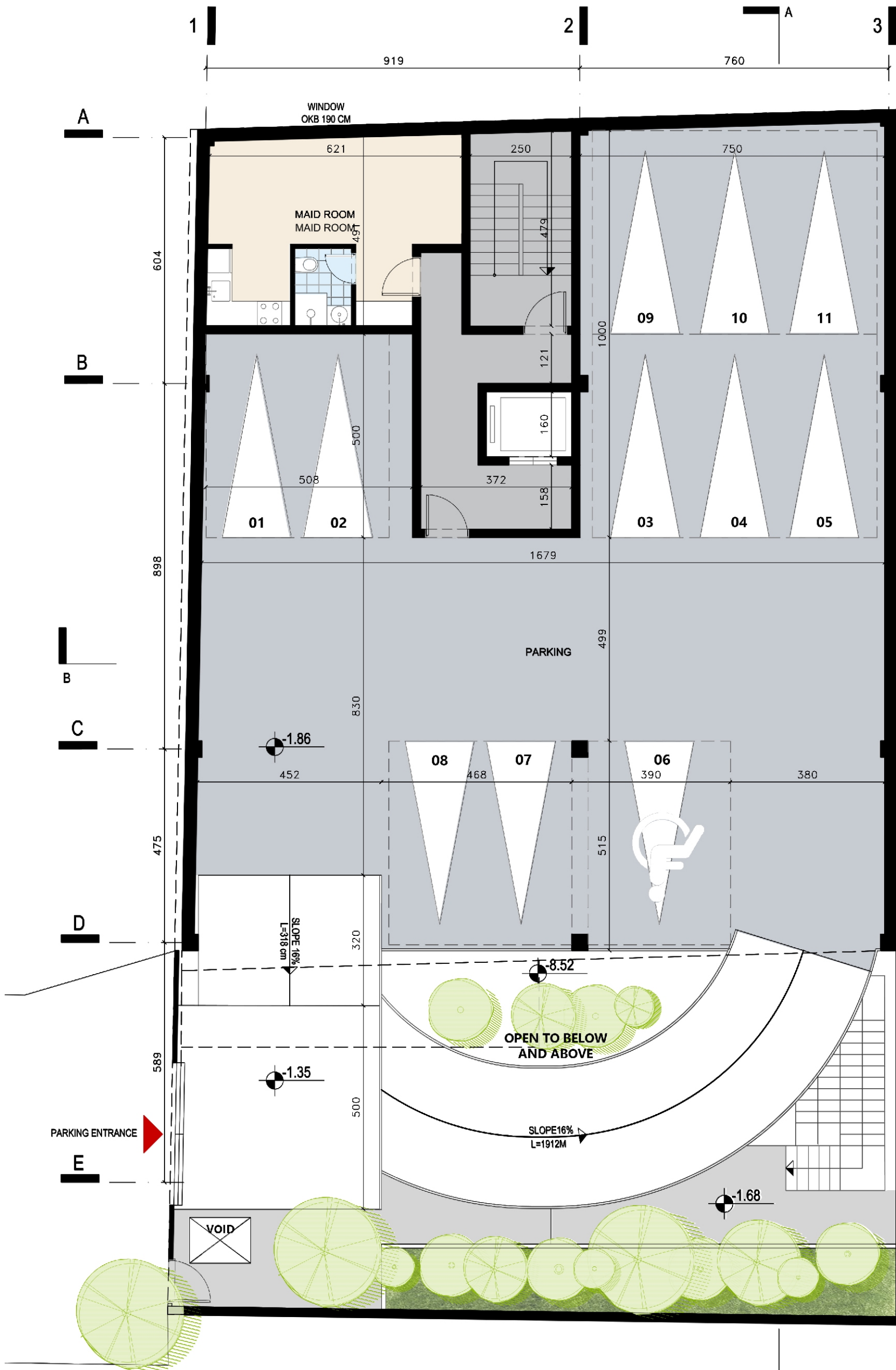
BASEMNET -1 | DIMENTION PLAN PARKING NO. 11
