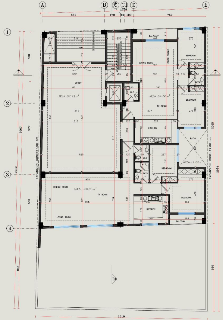
GROUND FLOOR PLAN SC. 1:100
