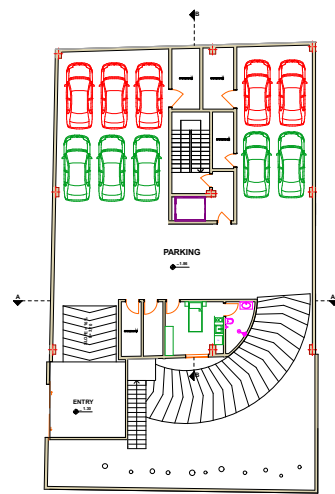
-1 BASEMENT PLAN
