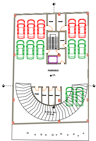
-2 BASEMENT PLAN
