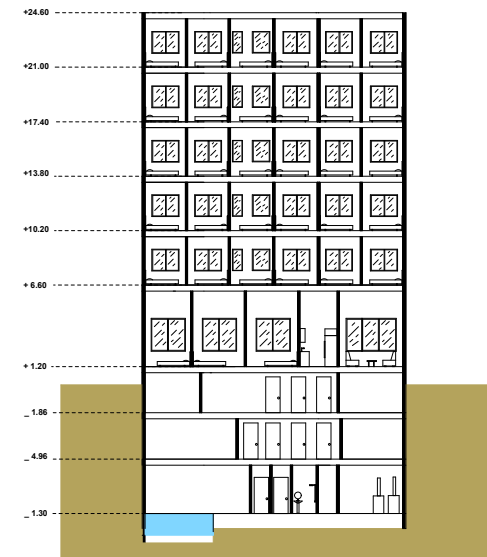
SECTION A-A SC 1/100
