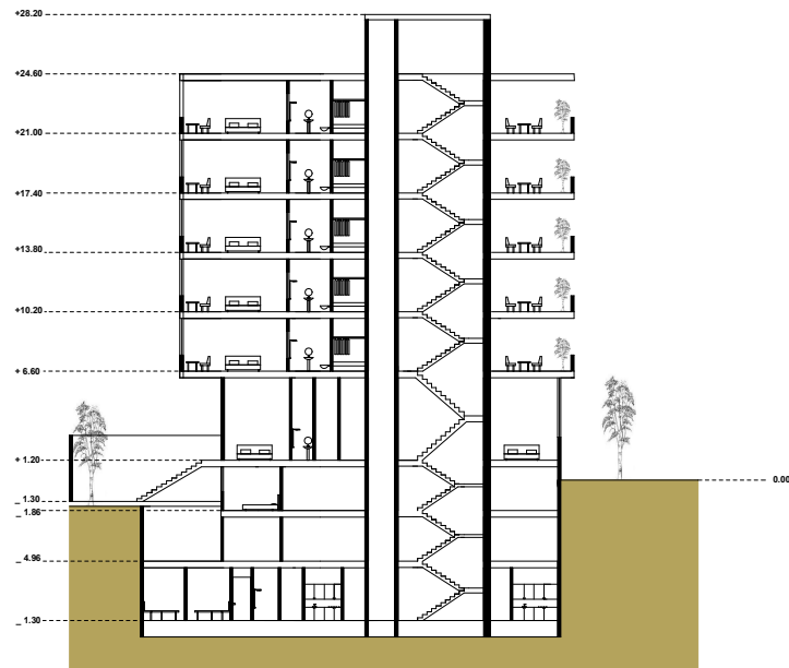
SECTION B-B SC 1/100
