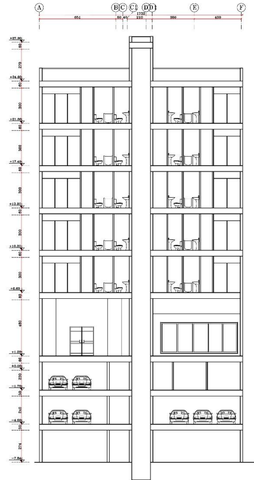
SECTION B-B SC. 1/100
