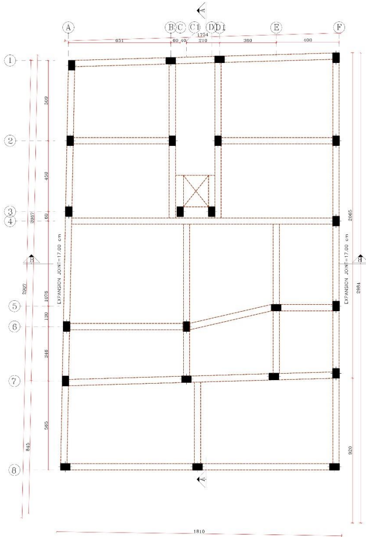
BASEMENT-3 FLOOR PLAN
