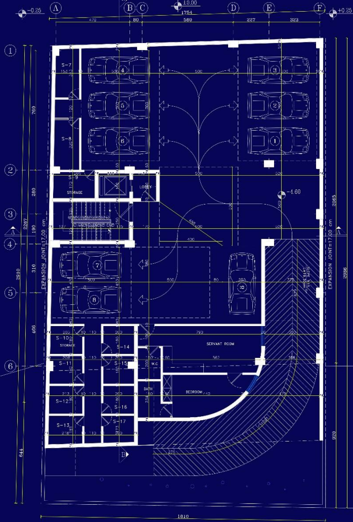
BASEMENT-2 FLOOR PLAN SC. 1:100
