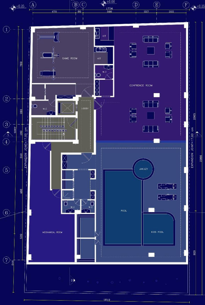
BASEMENT-3 FLOOR PLAN SC. 1:100
