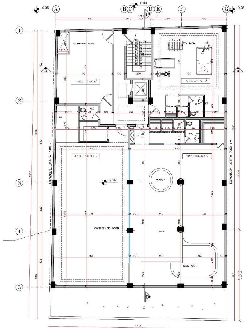
BASEMENT-3 FLOOR PLAN SC. 1:100
