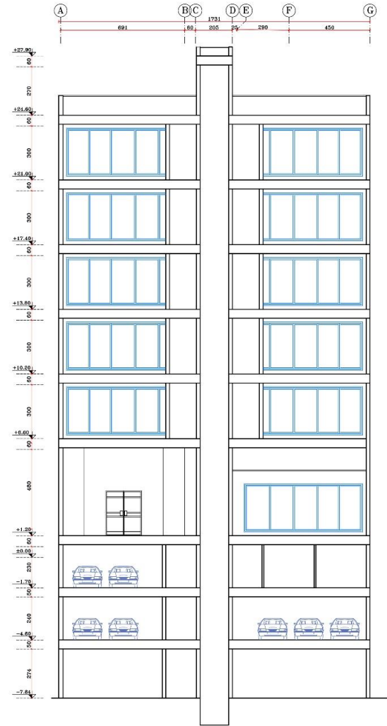
SECTION B-B SC. 1:100
