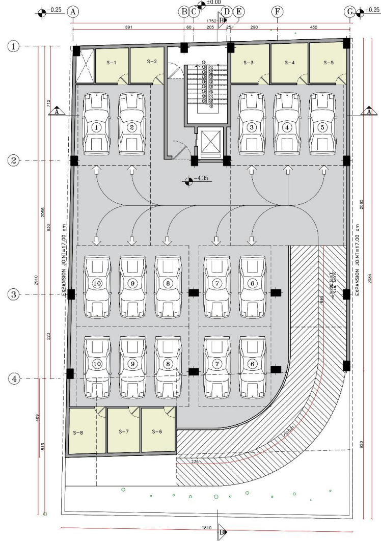
BASEMENT-2 FLOOR PLAN SC. 1:100
