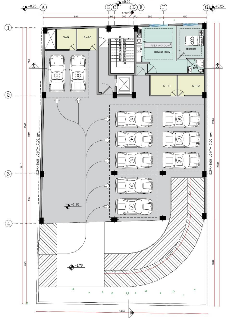
BASEMENT-1 FLOOR PLAN SC. 1:100
