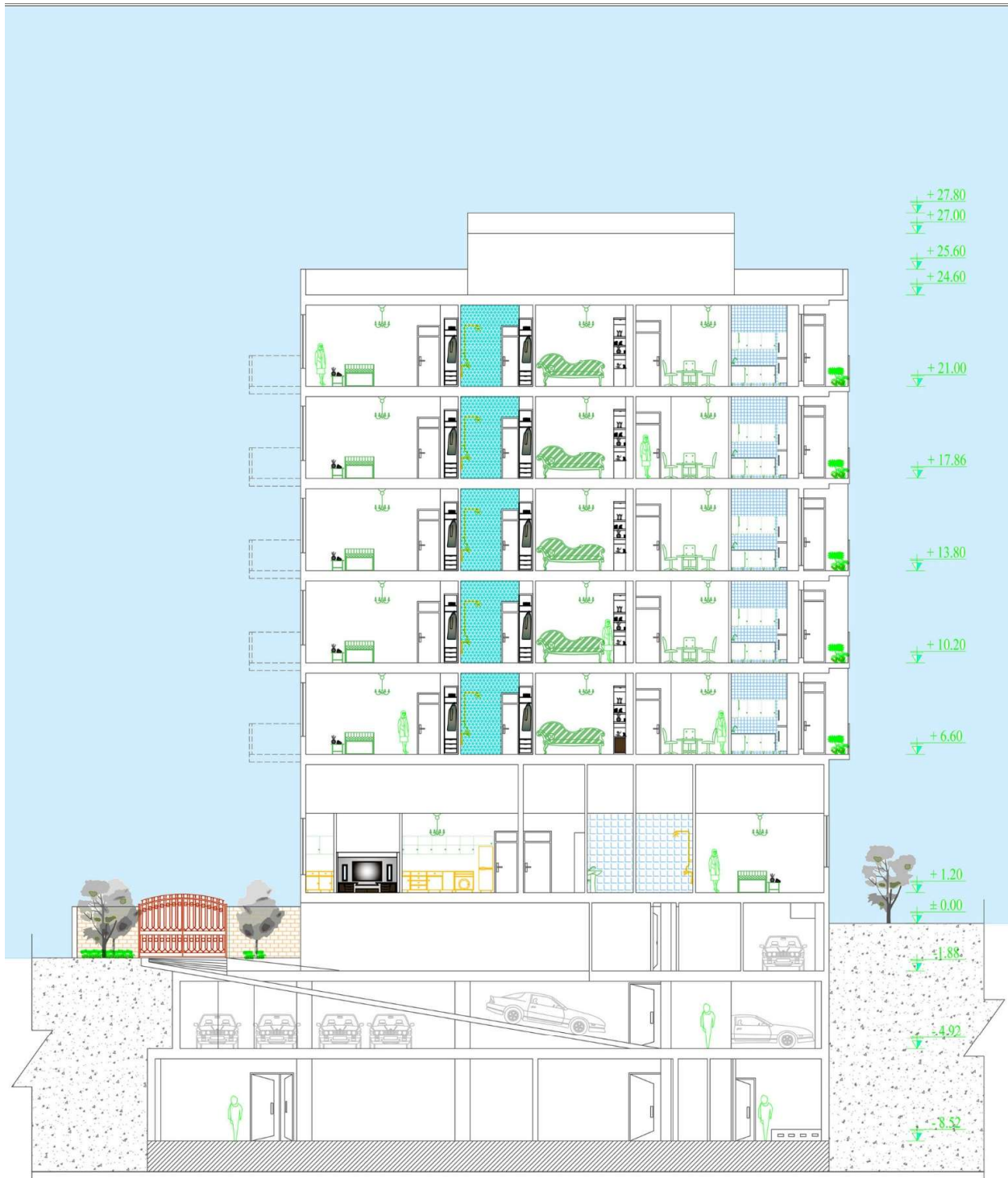
SECTION: A-A
