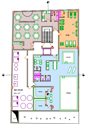
- 3 BASEMENT PLAN
