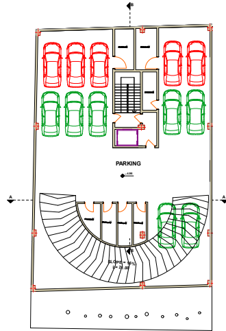
- 2 BASEMENT PLAN
