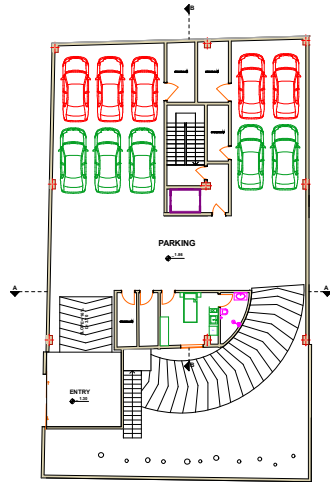
- 1 BASEMENT PLAN
