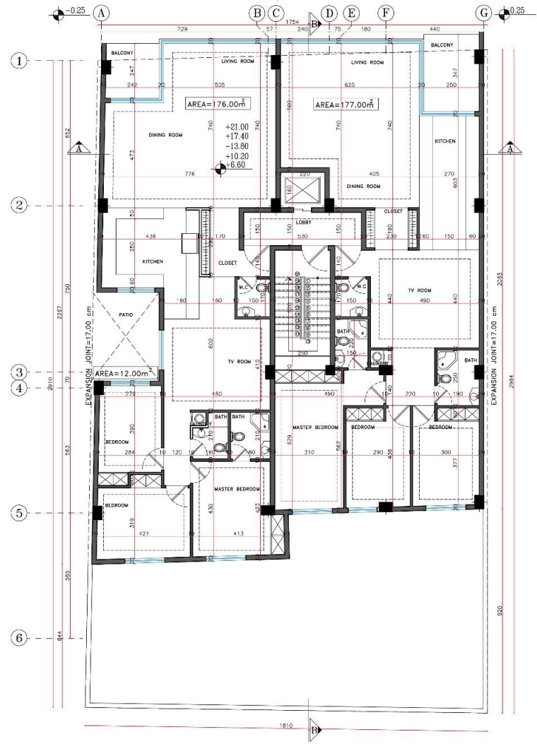
TYPICAL FLOORS PLAN SC. 1:100
