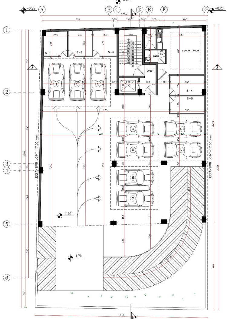
BASEMENT-1 FLOOR PLAN SC. 1:100
