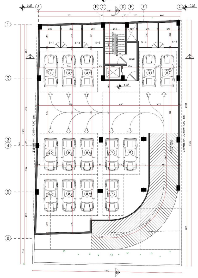
BASEMENT-2 FLOOR PLAN SC. 1:100
