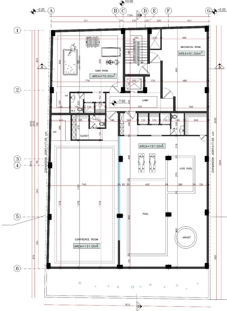
BASEMENT-3 FLOOR PLAN SC. 1:100
