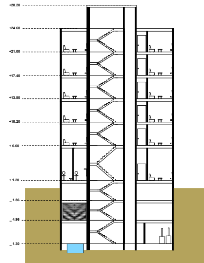
SECTION A-A SC 1/100
