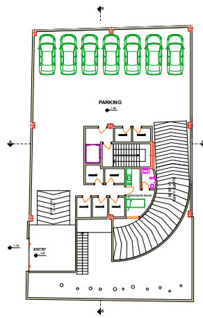
-1 BASEMENT PLAN
