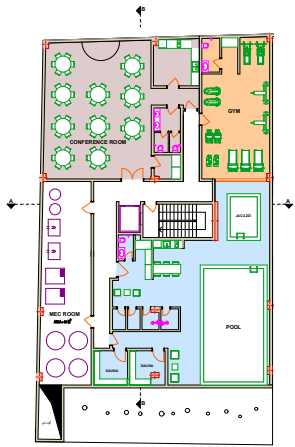
-3 BASEMENT PLAN
