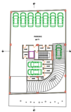
-2 BASEMENT PLAN
