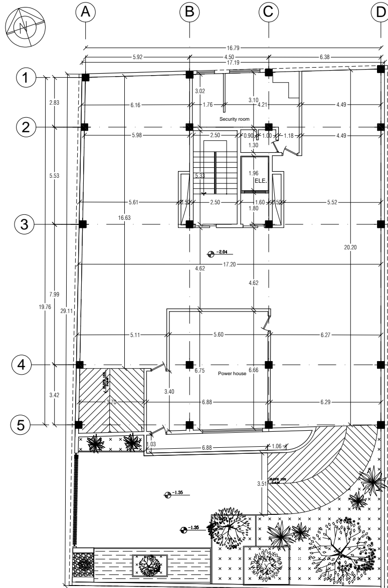
Parking -1 Dimension Plan
