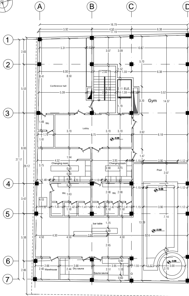
Parking -3 Dimension Plan
