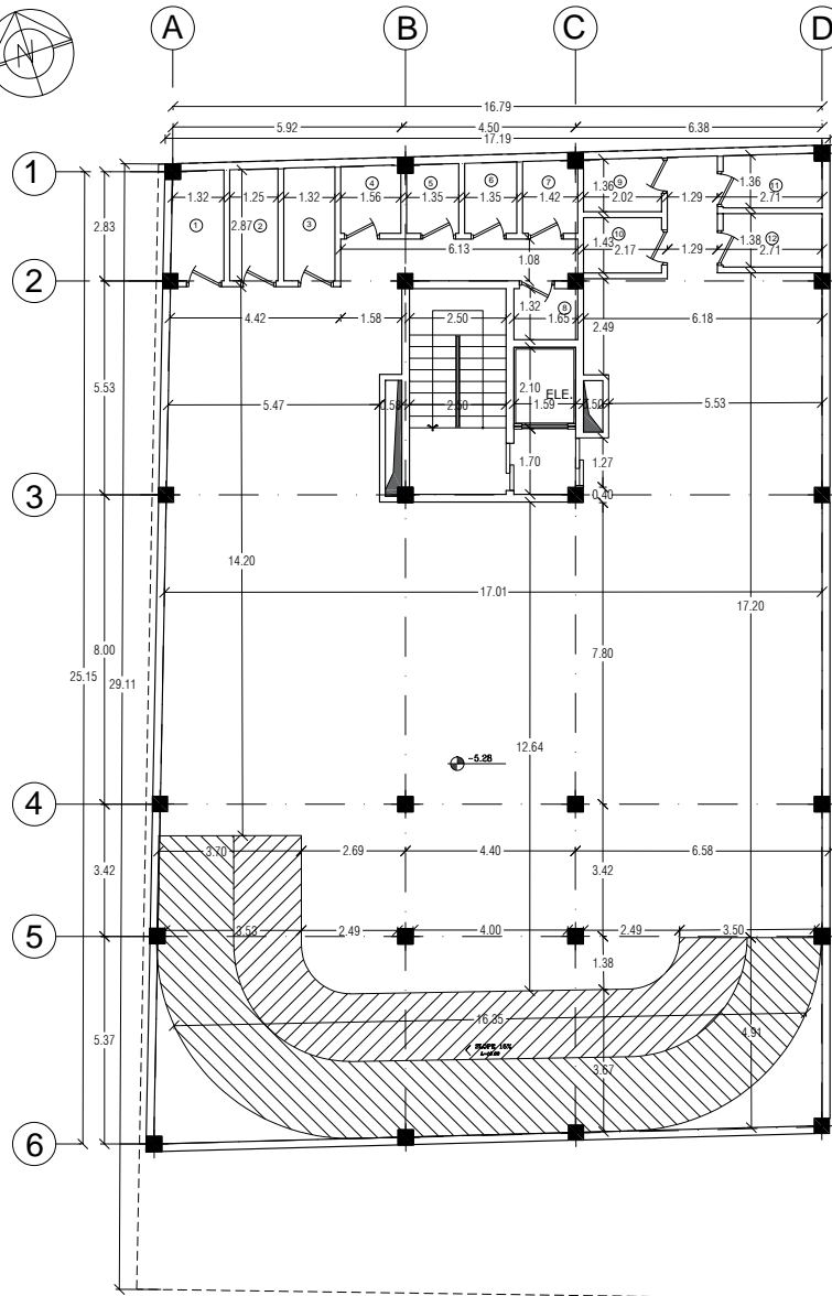
Parking -2 Dimension Plan
