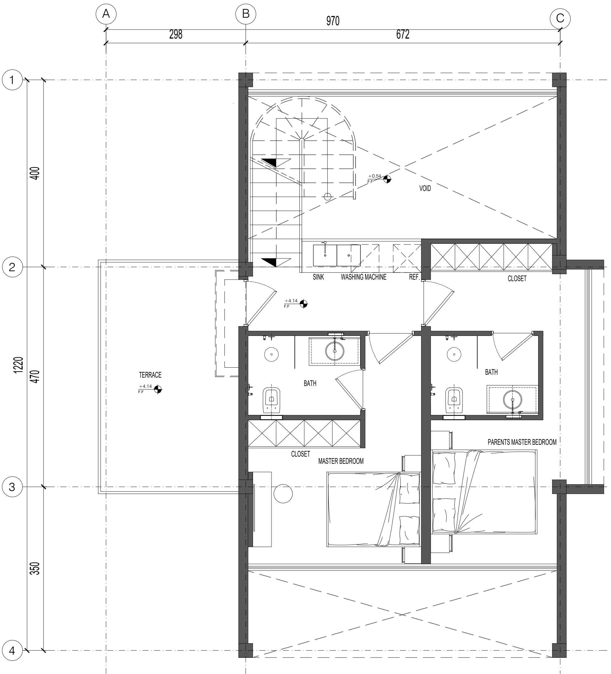
+1 FLOOR PLAN SCALE : 1:100
