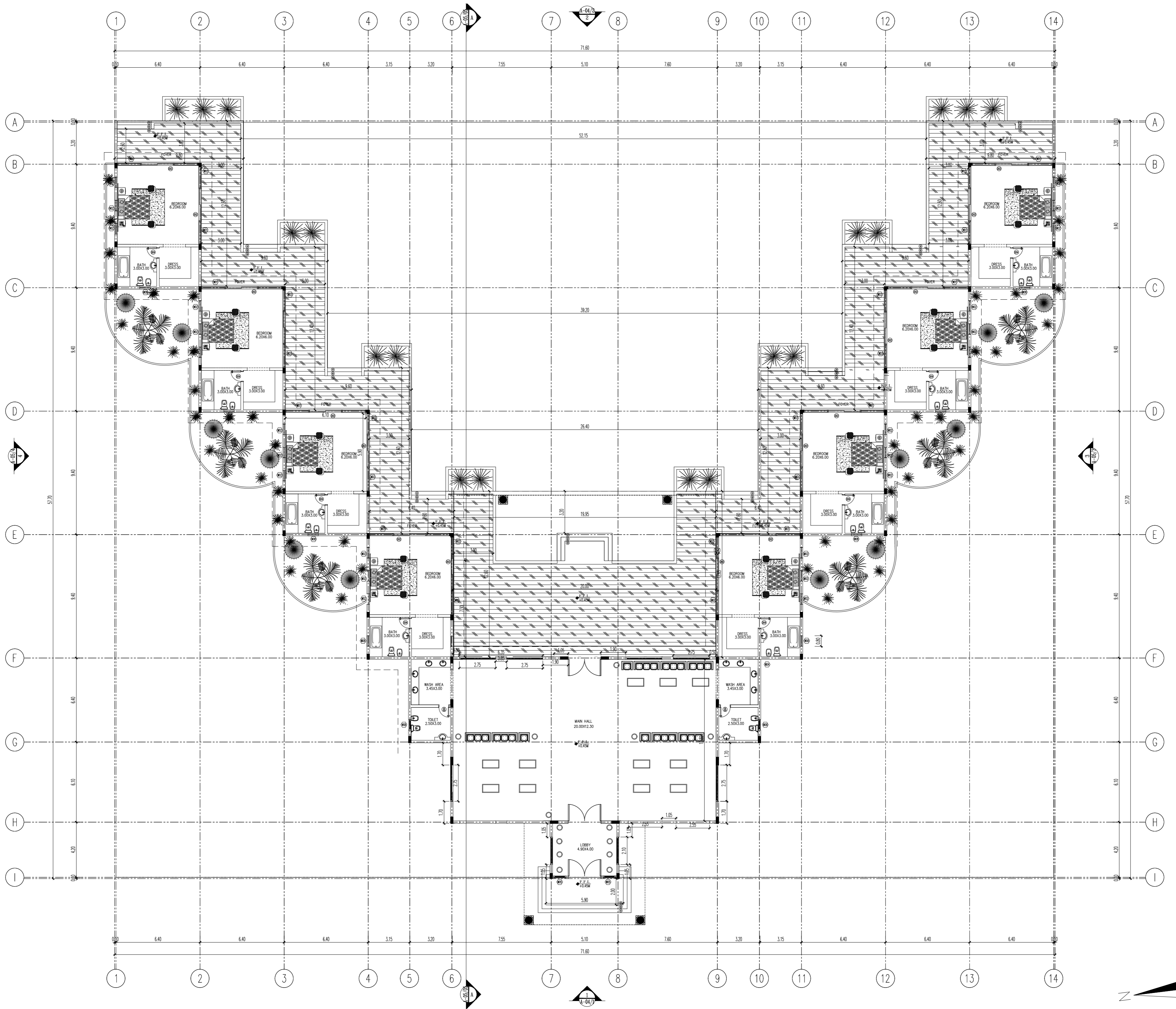
GROUND FLOOR PLAN (CHALET & MAILS) SCALE: 1:100
