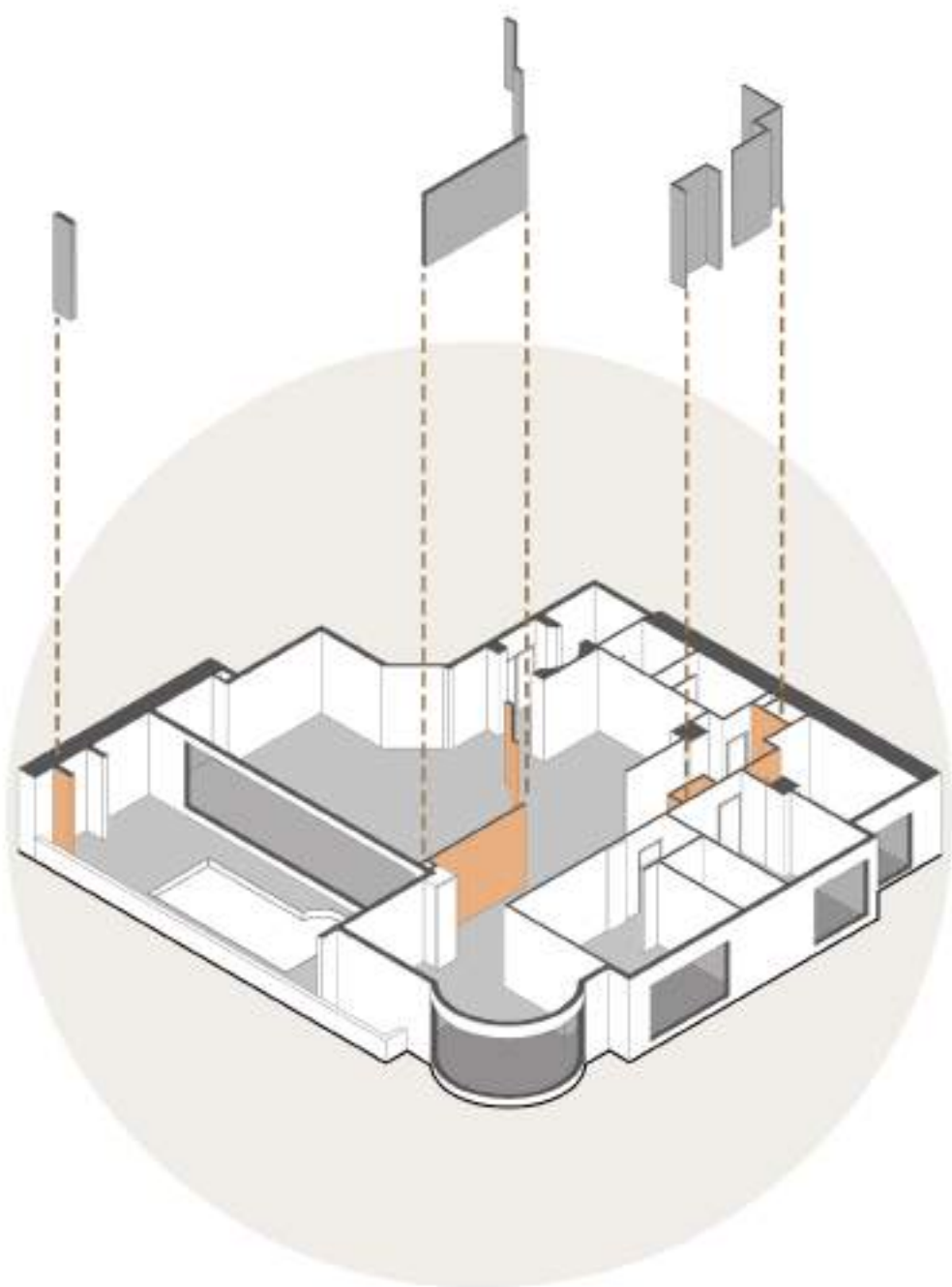
REMOVED WALLS
