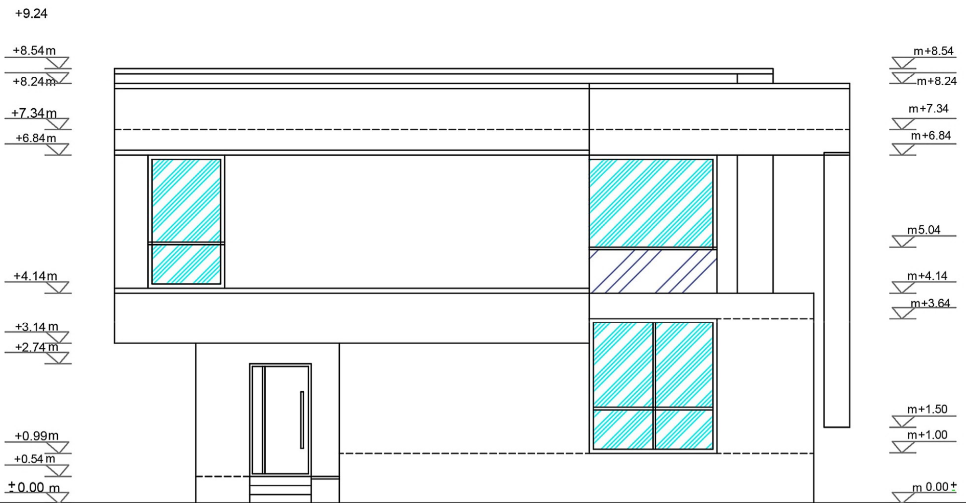
Northern-facade
